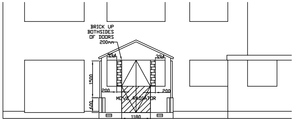
VENT THROUGH AIRBRICKS
